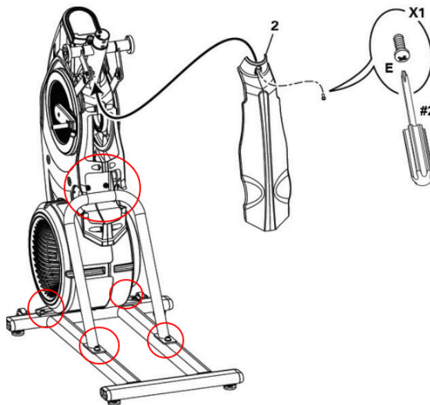
Remove the rear shroud as indicated in this image. The bolts to remove are circled in red.
