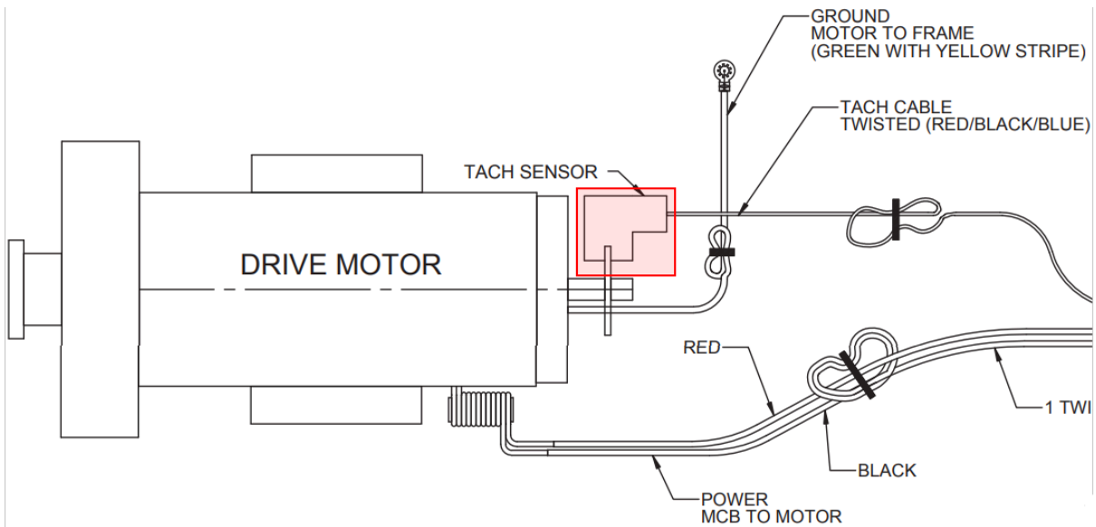
The tach sensor is located within the red box in the diagram above.
